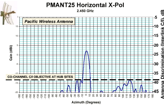
Grid Antenna X-Pol RPE (H-pol)
